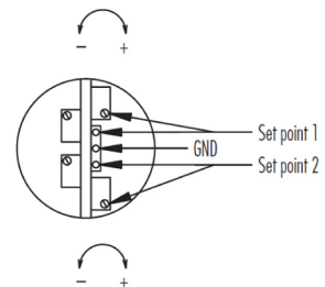
Connector side
